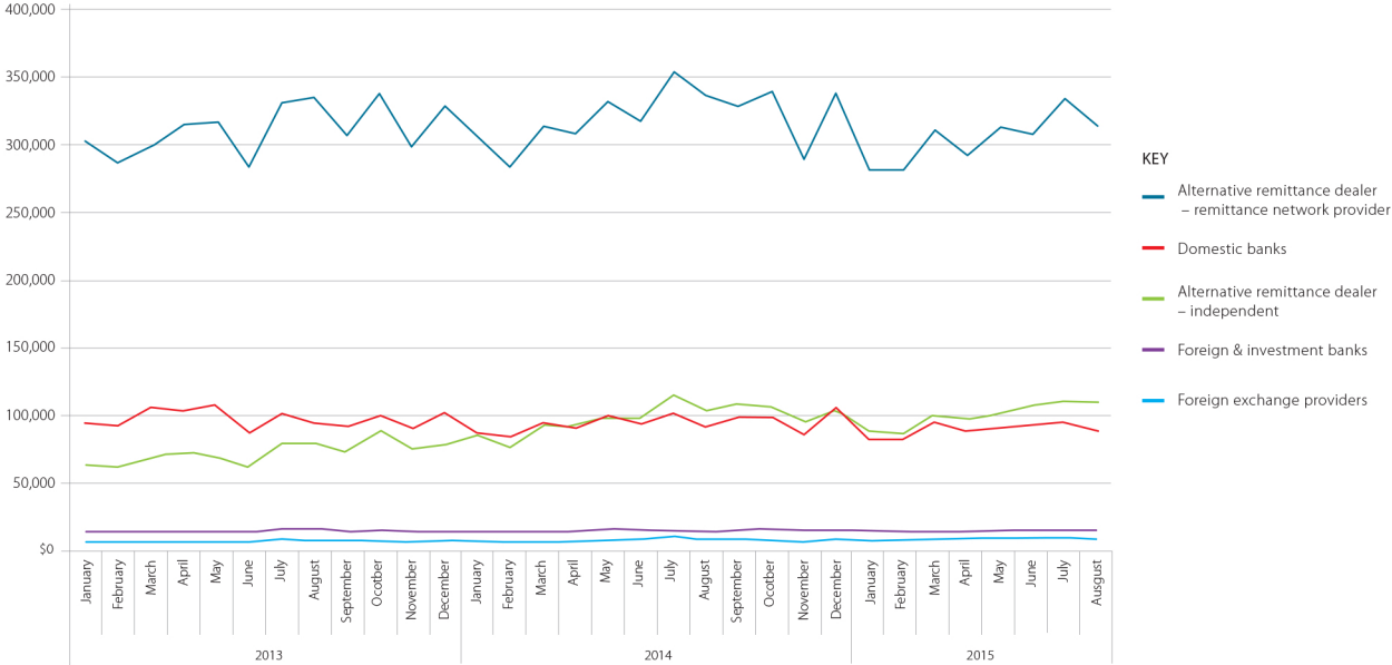
Figure 1– Report count - IFTIs out $500 or less by month by industry sector, 2010–2015
